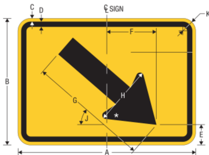
W16-7PR
