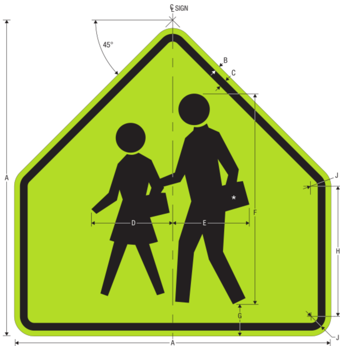
S1-1 SCHOOL
