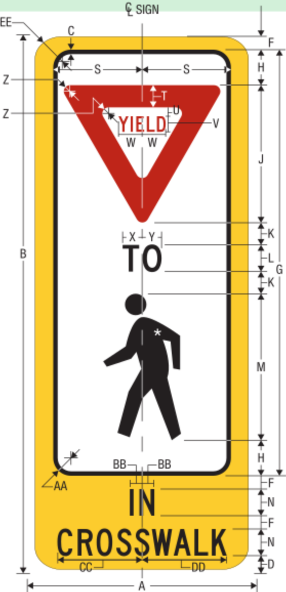
R1-6 IN-STREET PEDESTRIAN CROSSING - YIELD
