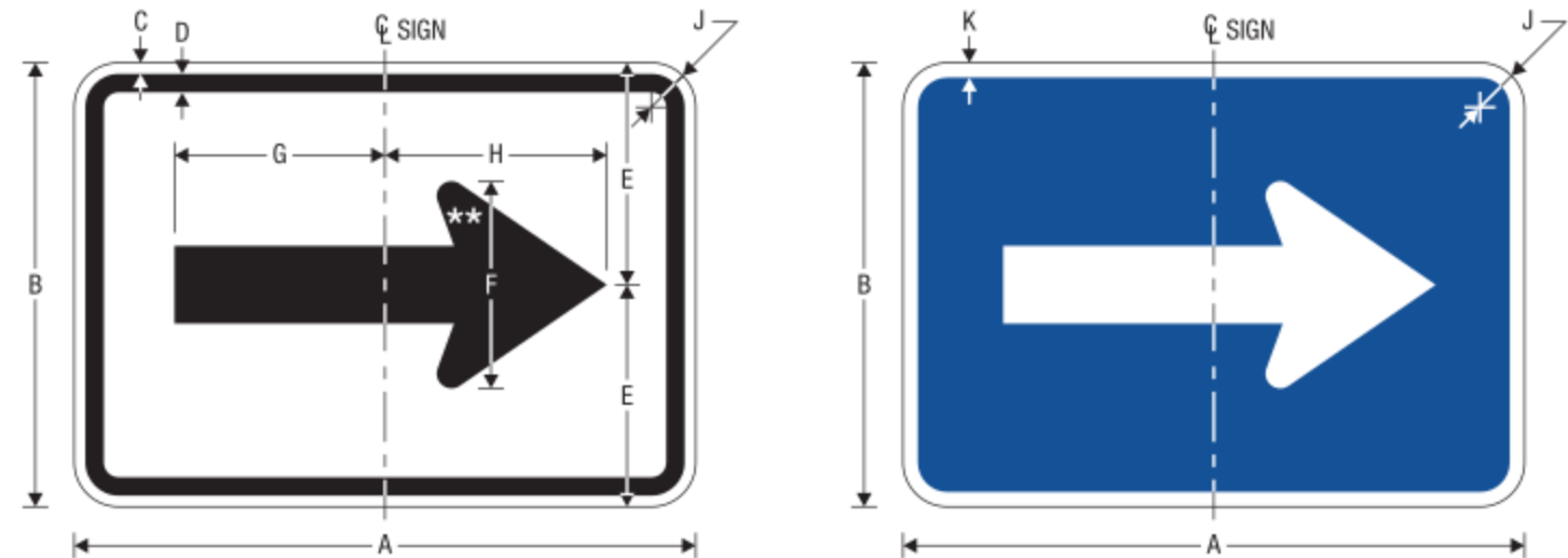
M6-1 DIRECTIONAL ARROW AUXILIARY
