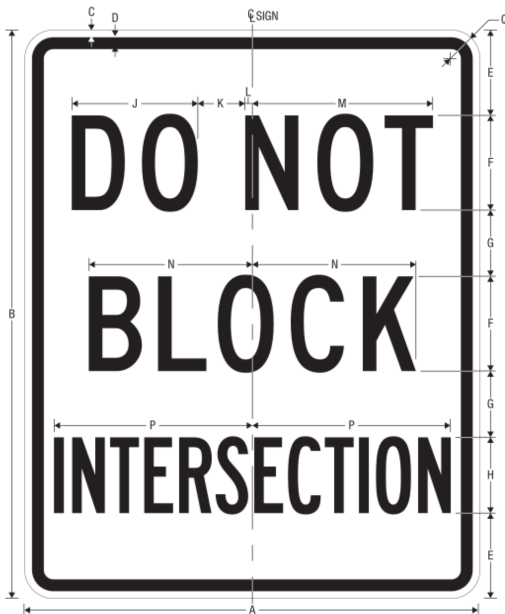
R10-7 DO NOT BLOCK INTERSECTION
