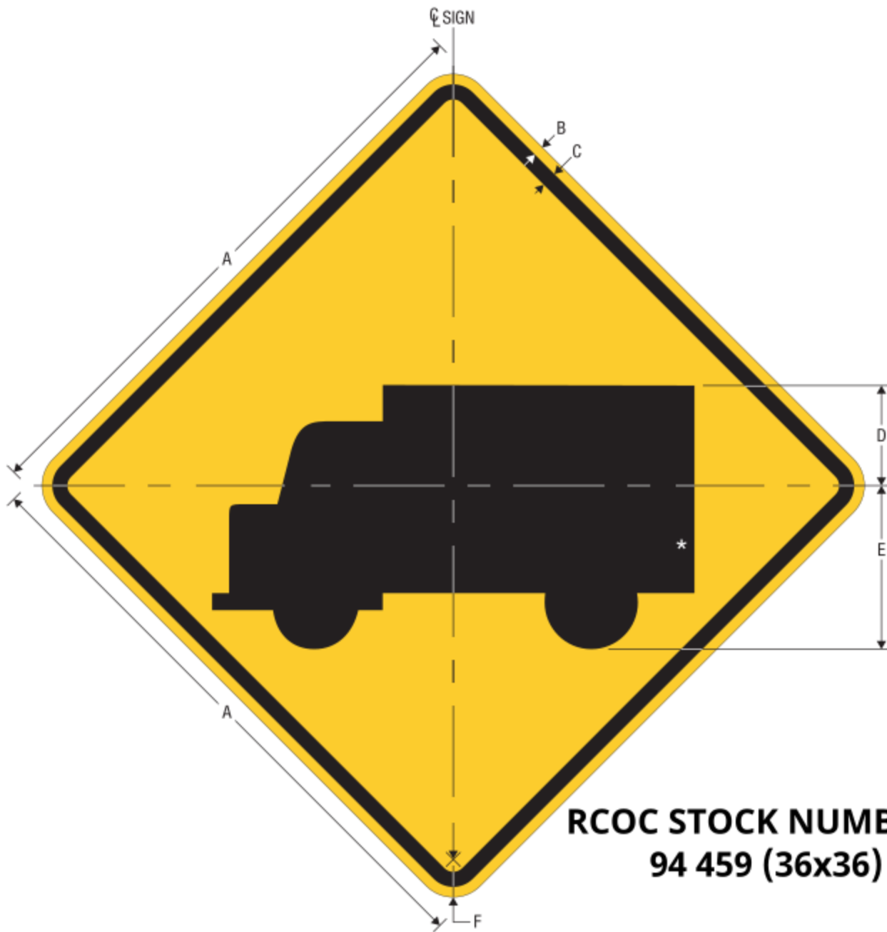
W11-10 TRUCK
