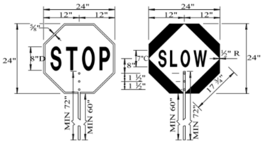
STAFF MOUNTED PADDLES
