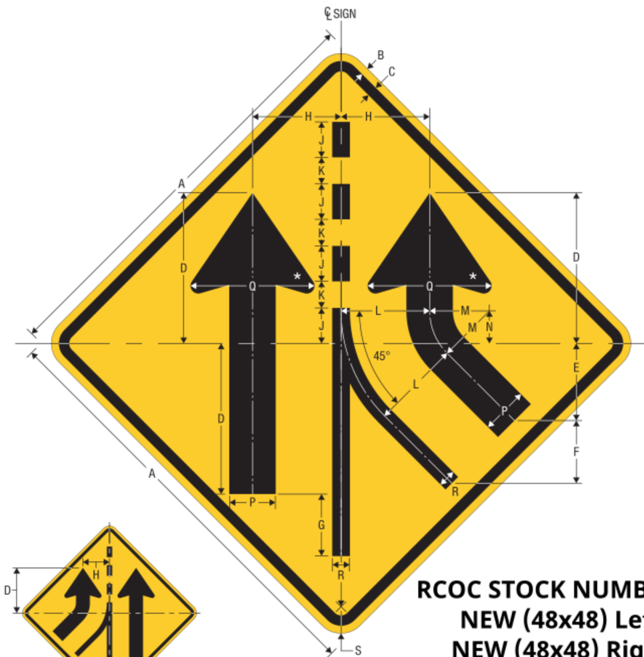
W4-3L W4-3R ADDED LANE
