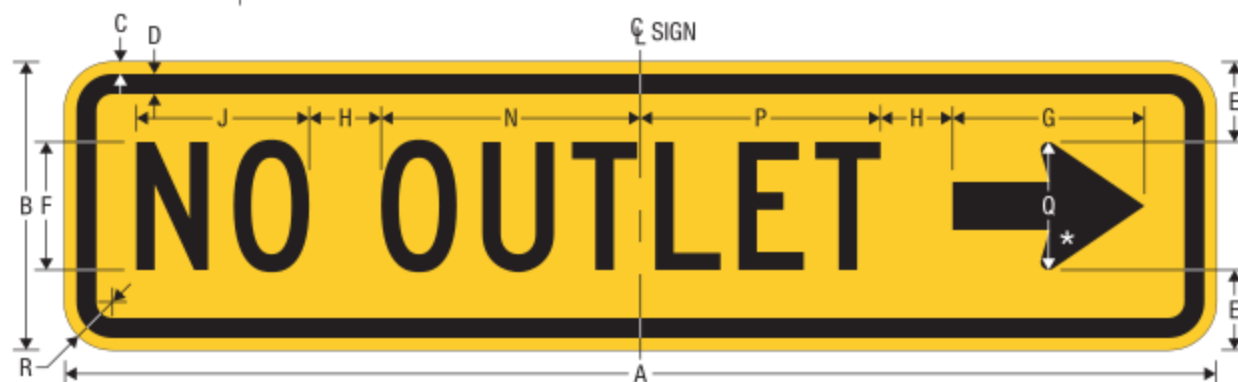
W14-2aR NO OUTLET (WITH ARROW)
