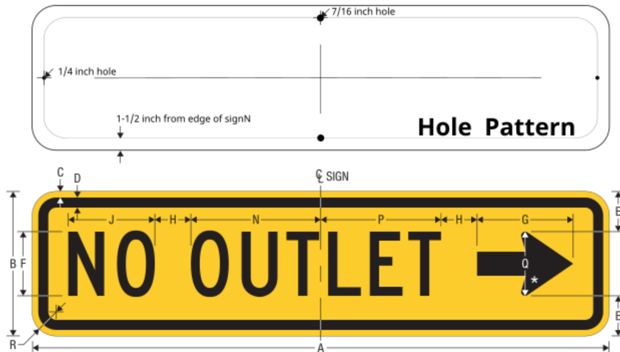
W14-2aR NO OUTLET (WITH ARROW)
